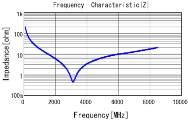
GRM1555C2A8R0DA01 |Z| DCOV, 25degC
