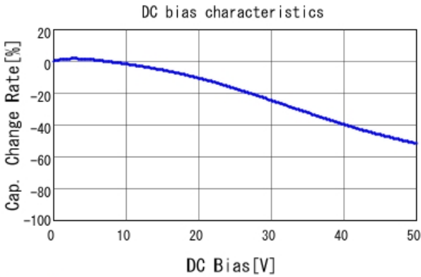
GRM21BR71H224KA01 C-DC bias capchange, 25.0degC, A
