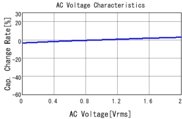
GRM21BR71H224KA01 C-AC Voltage capchange, DCOV, 25
