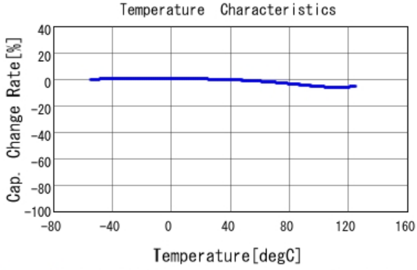
GRM21BR71H224KA01 C-Temp. capchange, DC0.0V, AC1.C
