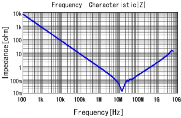
GRM21BR71H224KA01 |Z| DCOV, 25degC
