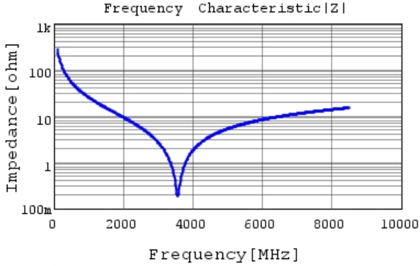
GCQ1555C1H5R8DB01 |Z| DC0V, 25degC
