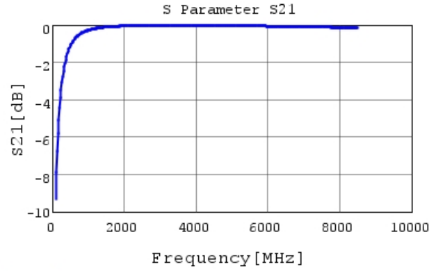
GCQ1555C1H5R8DB01 S21 DCOV, 25degC
