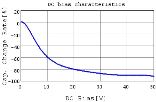
GRT188R61H225KE13 C-DC bias capchange, 25.0c
