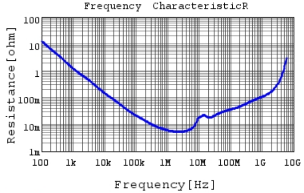
GRT188R61H225KE13 R DCOV, 25degC
