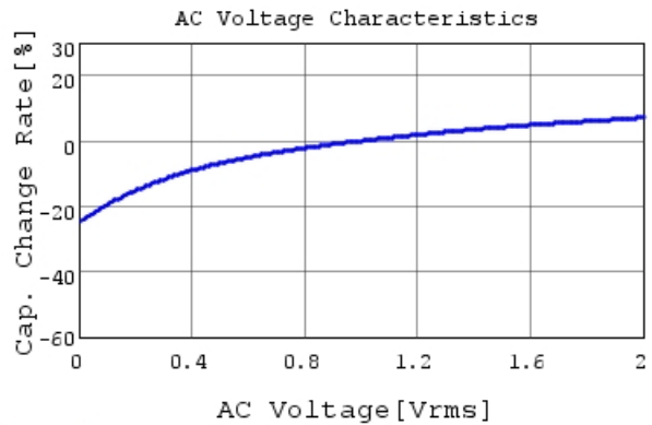
GRT188R61H225KE13 C-AC Voltage capchange, Dc
