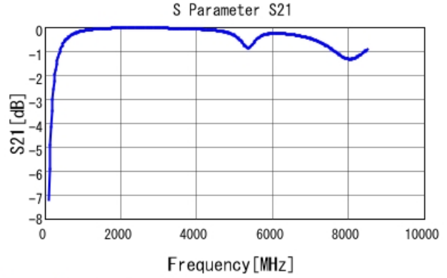
GRM1885C1H7R7WA01 S21 DCOV, 25degC
