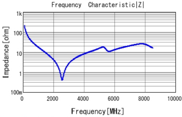
GRM1885C1H7R7WA01 |Z| DCOV, 25degC
