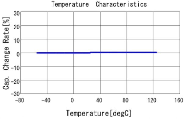
GRM1885C1H7R7WA01 C-Temp. capchange, DCOV, AC1Vrms
