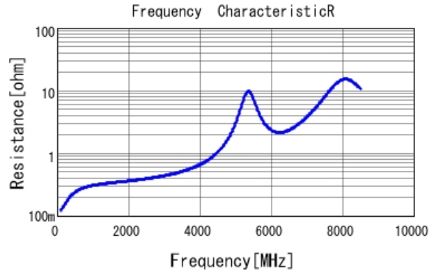
GRM1885C1H7R7WA01 R DCOV, 25degC
