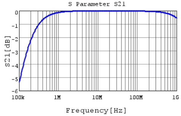
RDER73A103K2M1H03A S21 DCOV, 25degC
