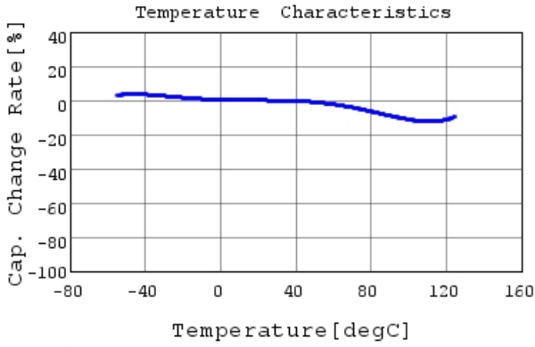
RDER73A103K2M1H03A C-Temp. capchange, DCOV,
