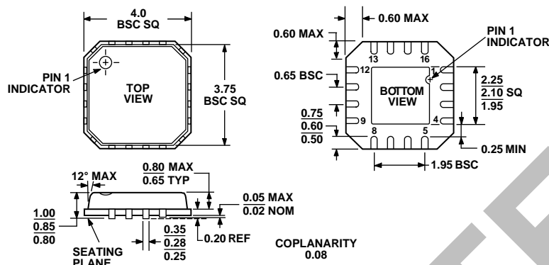
Figure 27. 4 × 4 mm 16-Lead Lead Frame Chip Scale Package [LFCSP] (CP-16)
