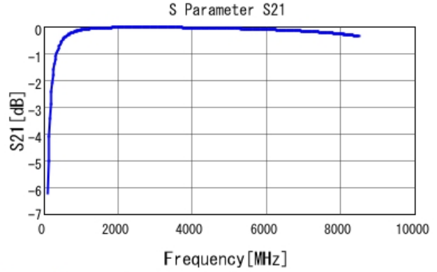
GRM0335C1H8R9CA01 S21 DCOV, 25degC
