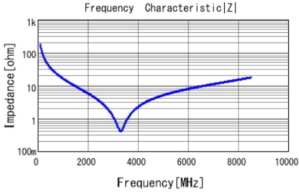
GRM0335C1H8R9CA01 |Z| DCOV, 25degC
