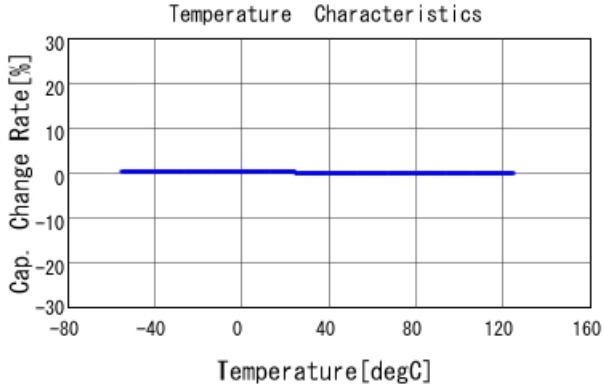
GRM0335C1H8R9CA01 C-Temp. capchange, DCOV, AC1Vrms
