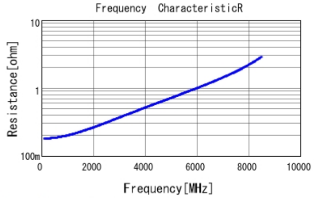
GRM0335C1H8R9CA01 R DCOV, 25degC
