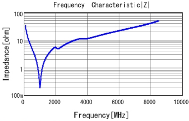
GCM1885C1H470JA16 |Z| DCOV, 25degC
