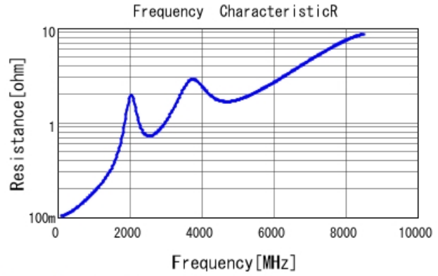
GCM1885C1H470JA16 R DCOV, 25degC
