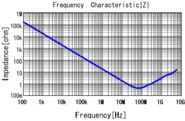
■ GCJ188R72A103MA01 |Z| DCOV, 25degC
