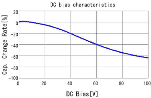
■ GCJ188R72A103MA01 C-DC bias capchange, 25.0degC, AC1.
