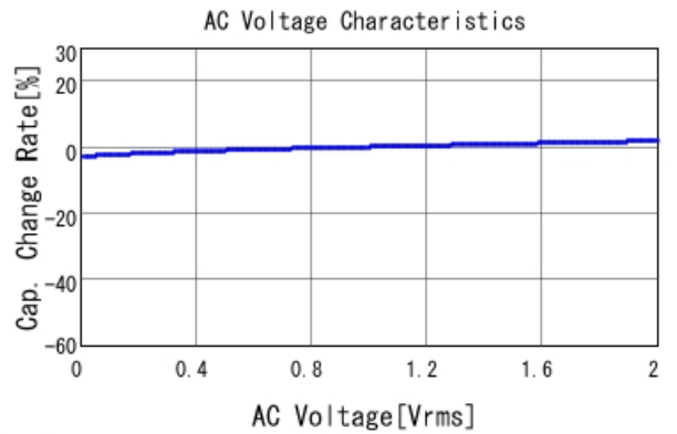
■ GCJ188R72A103MA01 C-AC Voltage capchange, DCOV, 25.0d
