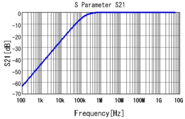
■ GCJ188R72A103MA01 S21 DCOV, 25degC
