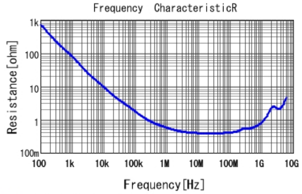
■ GCJ188R72A103MA01 R DCOV, 25degC
