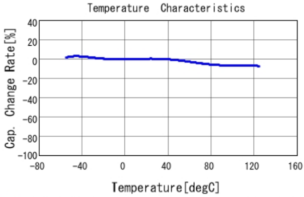
■ GCJ188R72A103MA01 C-Temp. capchange, DCO. 0V, AC1. 0Vrm
