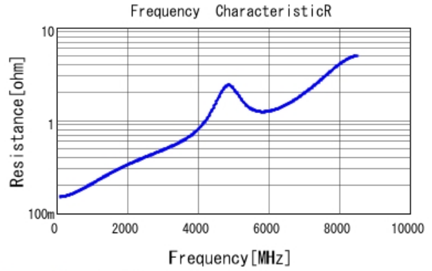
GRM1555C1H150GA01 R DCOV, 25degC
