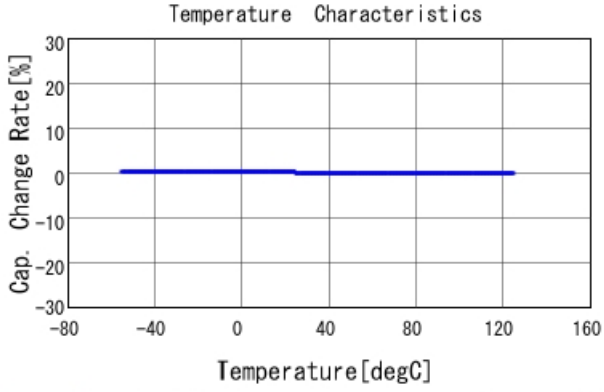
GRM1555C1H150GA01 C-Temp. capchange, DCOV, AC1Vrms
