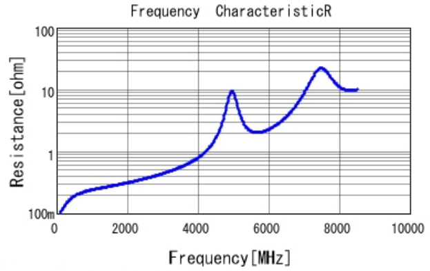
GRM1885C1H9R2DA01 R DCOV, 25degC
