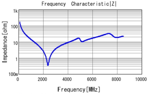
GRM1885C1H9R2DA01 |Z| DCOV, 25degC
