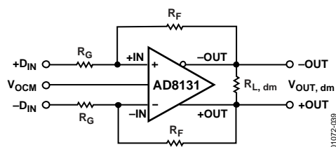
Figure 39. Circuit Definitions
