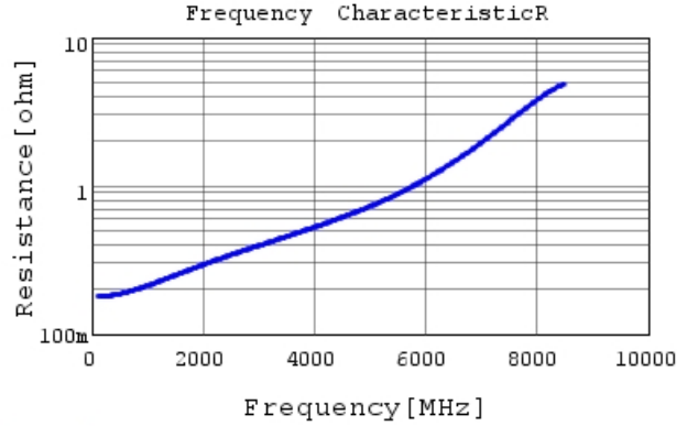
GRM0335C1H150GA01 R DCOV, 25degC
