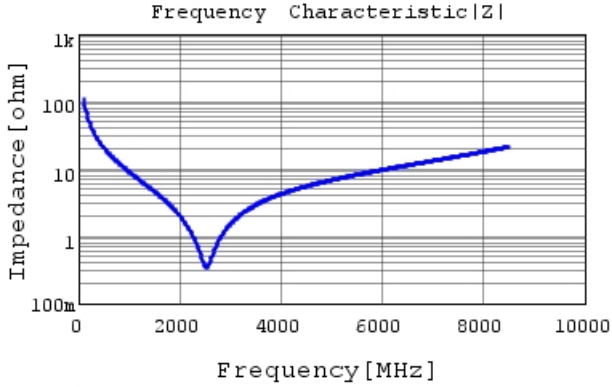
GRM0335C1H150GA01 |Z| DCOV, 25degC
