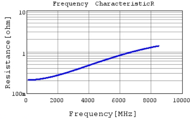
GRM0335C2A5R1BA01 R DCOV, 25degC
