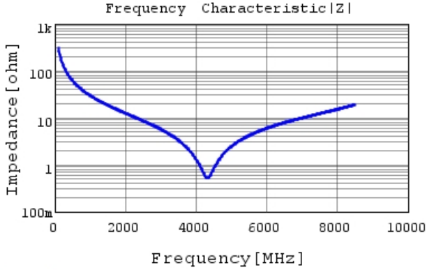
GRM0335C2A5R1BA01 |Z| DCOV, 25degC
