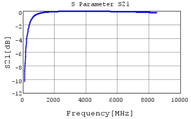
GRM0335C2A5R1BA01 S21 DCOV, 25degC
