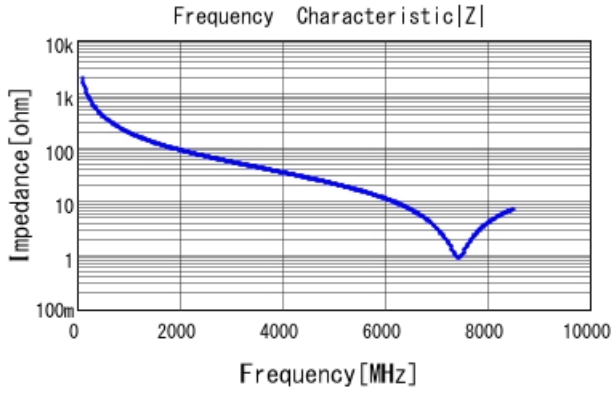
GRM1885C2AR80WA01 |Z| DCOV, 25degC
