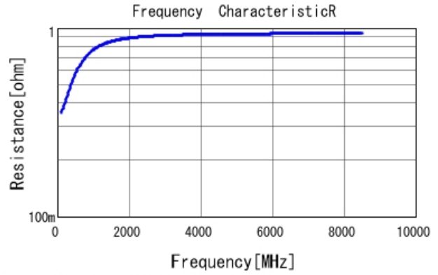
GRM1885C2AR80WA01 R DCOV, 25degC
