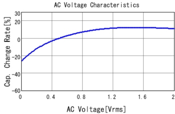
GRM188R60J475KE19 C-AC Voltage capchange, DCOV, 25
