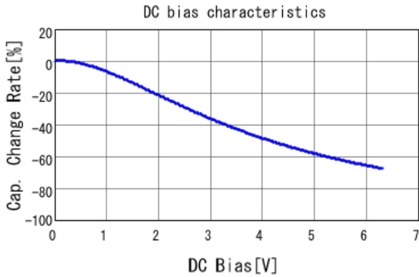
GRM188R60J475KE19 C-DC bias capchange, 25.0degC, A
