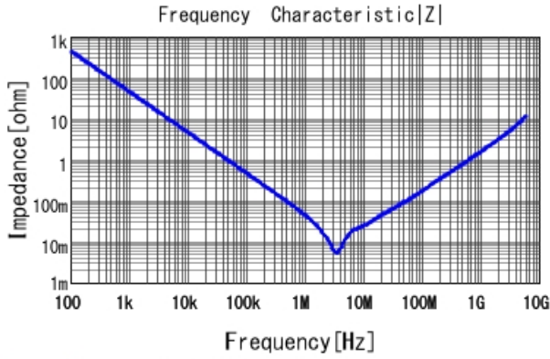
GRM188R60J475KE19 |Z| DCOV, 25degC
