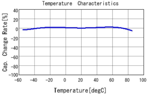
GRM188R60J475KE19 C-Temp. capchange, DC0.0V, AC0.5
