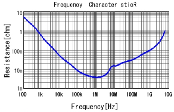
GRM188R60J475KE19 R DCOV, 25degC
