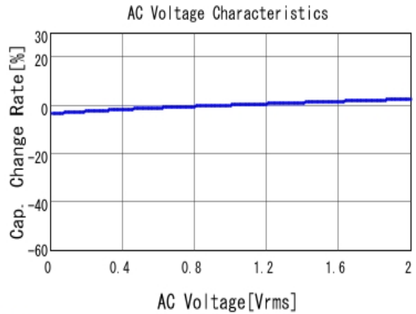
■ GRJ32EC71H106ME11 C-AC Voltage capchange, DCOV, 25.0d
