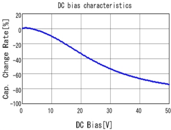
■ GRJ32EC71H106ME11 C-DC bias capchange, 25.0degC, AC1.
