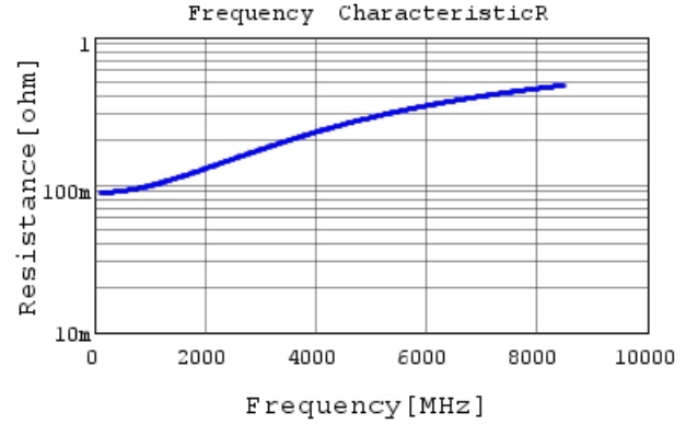
GCQ1555C1H6R7DB01 R DC0V, 25degC
