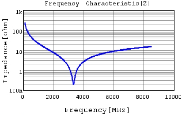
GCQ1555C1H6R7DB01 |Z| DC0V, 25degC
