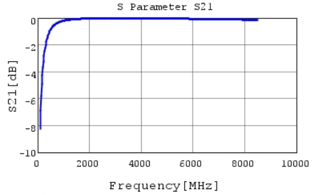
GCQ1555C1H6R7DB01 S21 DCOV, 25degC
