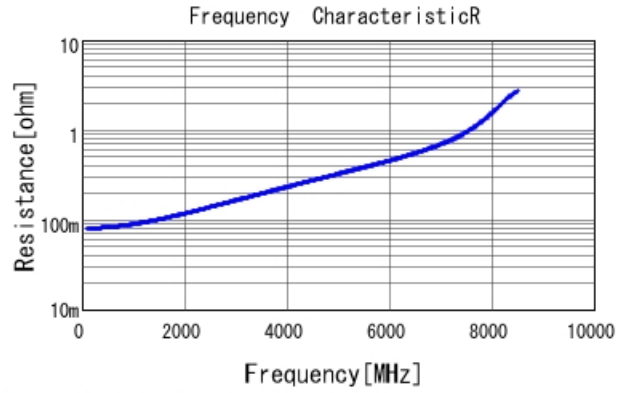
GCQ1555C1H7R1WB01 R DCOV, 25degC
