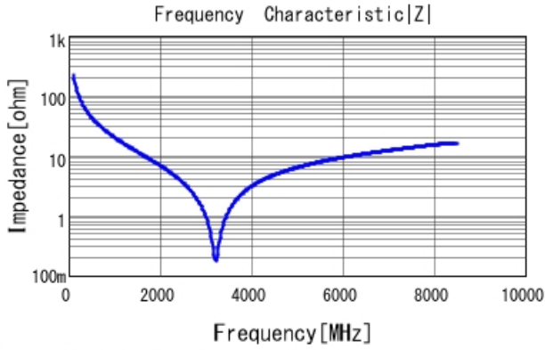
GCQ1555C1H7R1WB01 |Z| DCOV, 25degC
