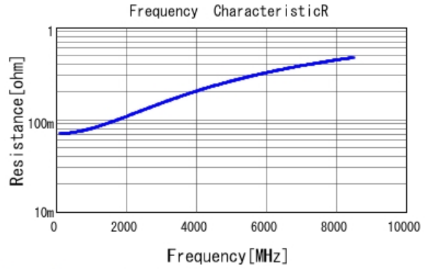
GJM0335C1E5R8WB01 R DCOV, 25degC
