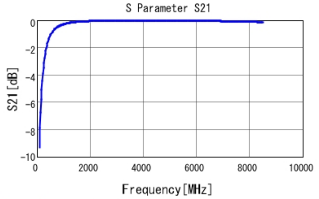
GJM0335C1E5R8WB01 S21 DC0V, 25degC
