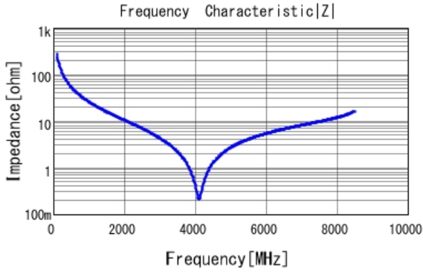
GJM0335C1E5R8WB01 |Z| DCOV, 25degC
