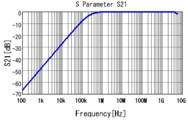
■ GCD188R71H682MA01 S21 DCOV, 25degC
