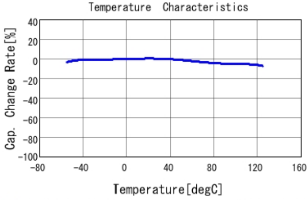
■ GCD188R71H682MA01 C-Temp. capchange, DCO. 0V, AC1. 0Vrm
