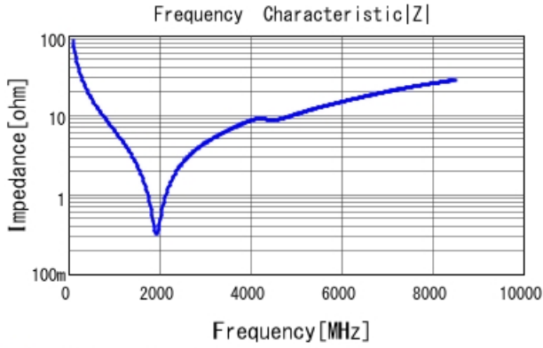
GRT1555C1E180JA02 |Z| DCOV, 25degC
