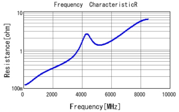
GRT1555C1E180JA02 R DCOV, 25degC
