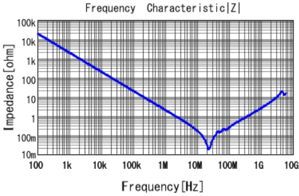
■ GCD21BR72A823MA01 |Z| DCOV, 25degC
