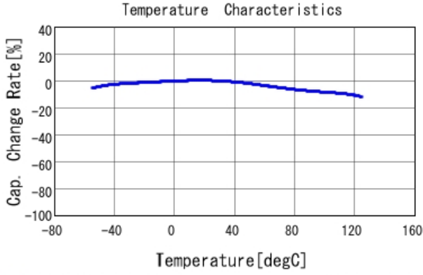
■ GCD21BR72A823MA01 C-Temp. capchange, DCO. 0V, AC1. 0Vrm
