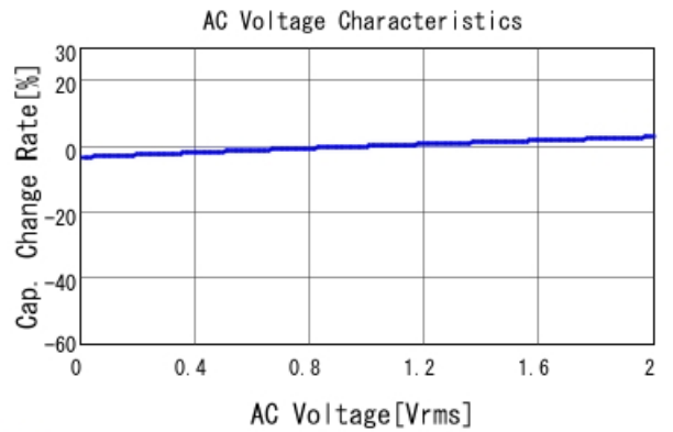
■ GCD21BR72A823MA01 C-AC Voltage capchange, DCOV, 25.0d
