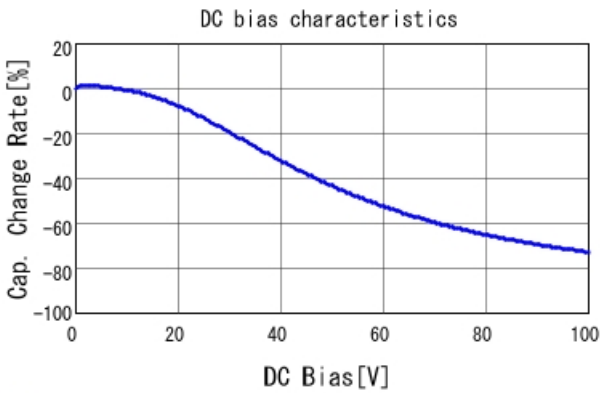
■ GCD21BR72A823MA01 C-DC bias capchange, 25.0degC, AC1.
