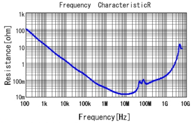
■ GCD21BR72A823MA01 R DCOV, 25degC
