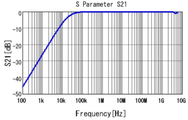
■ GCD21BR72A823MA01 S21 DCOV, 25degC
