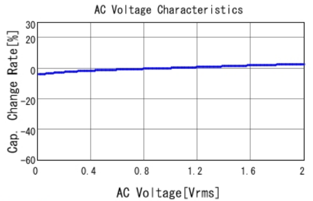
GRM21BR71E224KA01 C-AC Voltage capchange, DCOV, 25
