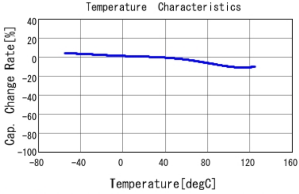
GRM21BR71E224KA01 C-Temp. capchange, DC0.0V, AC1.C
