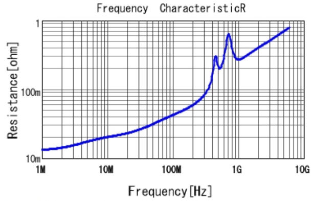
GRT1885C1E122JA02 R DCOV, 25degC
