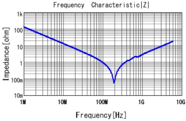
GRT1885C1E122JA02 |Z| DCOV, 25degC
