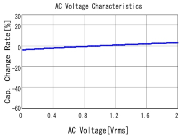
■ GCE188R71E273KA01 C-AC Voltage capchange, DCOV, 25.0d
