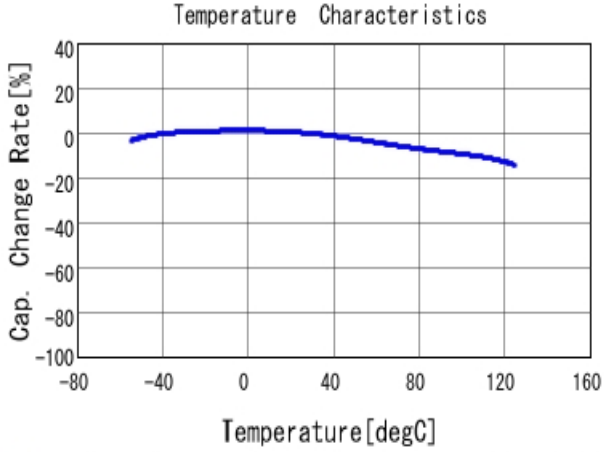
■ GCE188R71E273KA01 C-Temp. capchange, DC0.0V, AC1.0V r m
