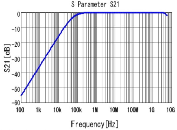
■ GCE188R71E273KA01 S21 DC0V, 25degC
