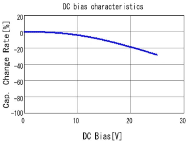
■ GCE188R71E273KA01 C-DC bias capchange, 25.0degC, AC1.
