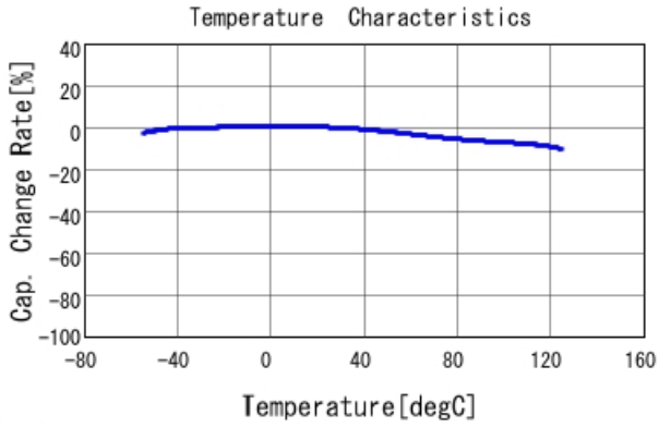
■ GCD188R72A183KA01 C-Temp. capchange, DCO. 0V, AC1. 0Vrm
