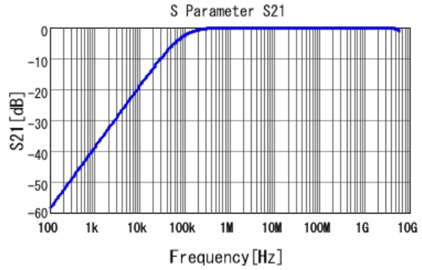
■ GCD188R72A183KA01 S21 DCOV, 25degC
