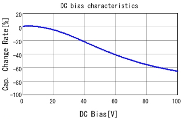
GCD188R72A183KA01 C-DC bias capchange, 25.0degC, AC1.
