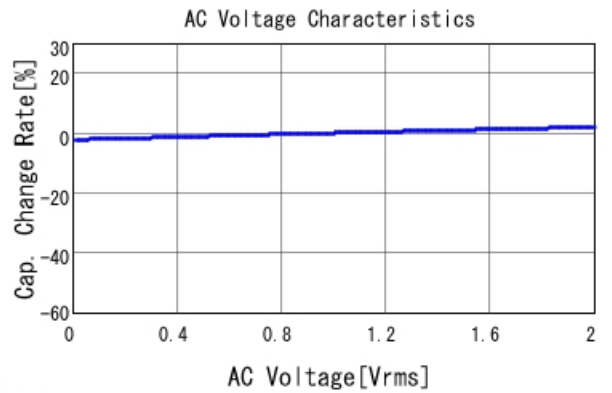
GCD188R72A183KA01 C-AC Voltage capchange, DCOV, 25.0d
