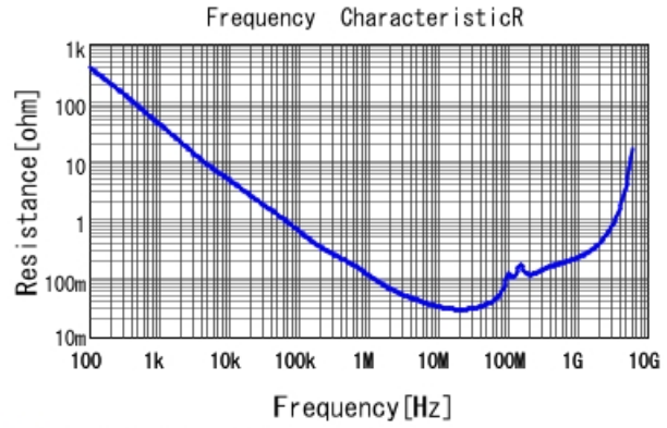
GCD188R72A183KA01 R DCOV, 25degC
