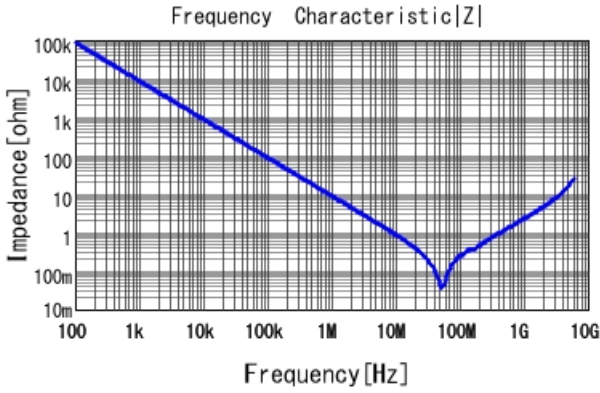
GCD188R72A183KA01 |Z| DCOV, 25degC
