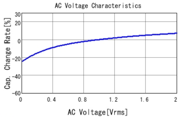
■ GRM188C81E225KE11 C-AC Voltage capchange, DCOV, 25.0d
