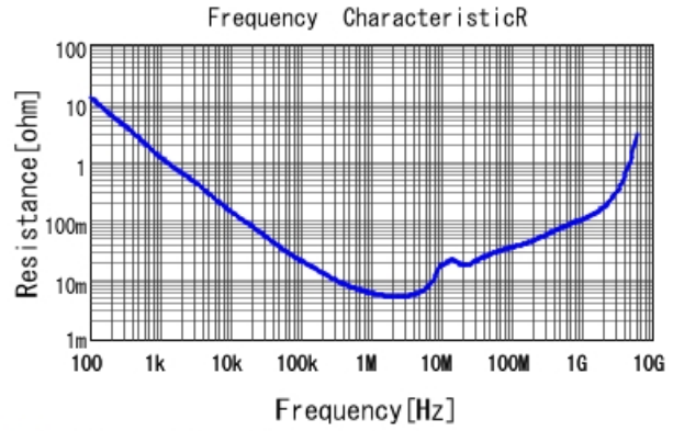
■ GRM188C81E225KE11 R DCOV, 25degC
