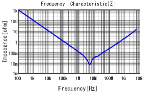
■ GRM188C81E225KE11 |Z| DCOV, 25degC
