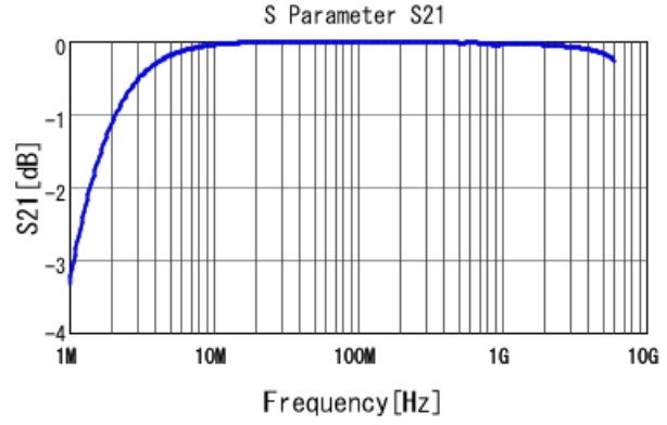
GRM2165C1H152JA01 S21 DCOV, 25degC
