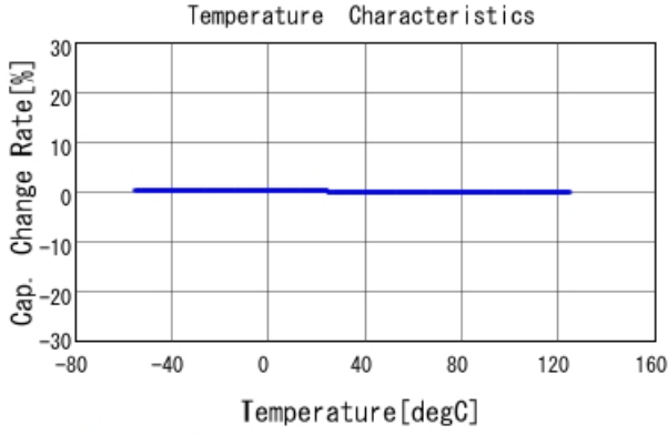
GRM2165C1H152JA01 C-Temp. capchange, DCOV, AC1Vrms
