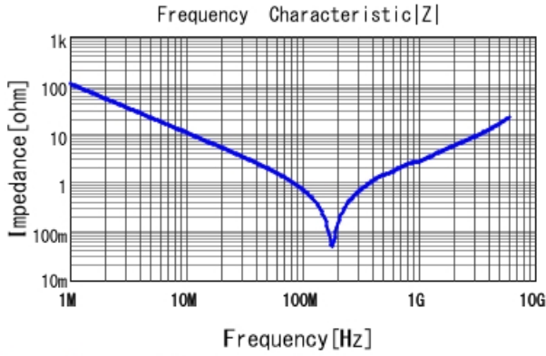
GRM2165C1H152JA01 |Z| DCOV, 25degC
