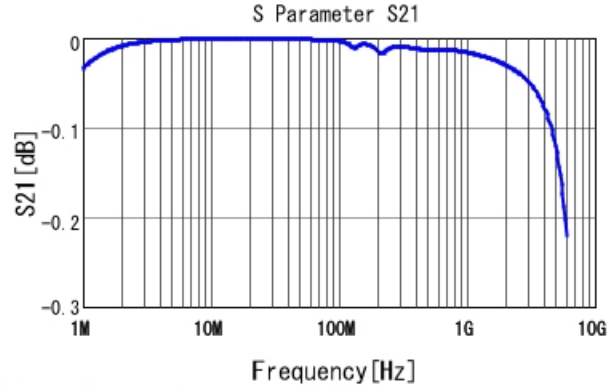
GRM2165C1H183JA01 S21 DCOV, 25degC
