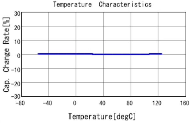
GRM2165C1H183JA01 C-Temp. capchange, DCOV, AC1Vrms
