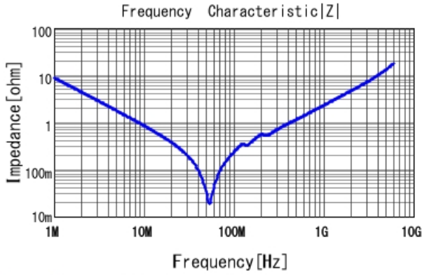
GRM2165C1H183JA01 |Z| DCOV, 25degC
