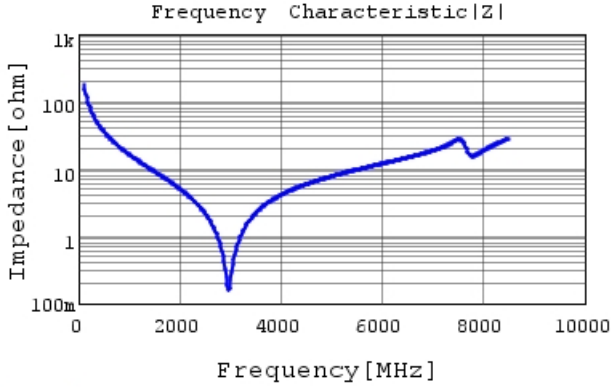
GCQ1555C1H8R7CB01 |Z| DC0V, 25degC
