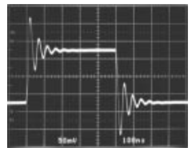
Small-Signal Transient ( A_V = -1, C_L = 200pF )
