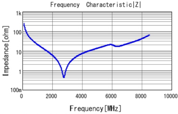
GRM1885C1H6R6WA01 |Z| DCOV, 25degC
