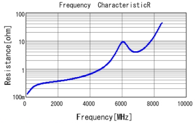
GRM1885C1H6R6WA01 R DCOV, 25degC
