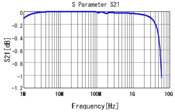
GRM3192C1H103JA01 S21 DCOV, 20degC
