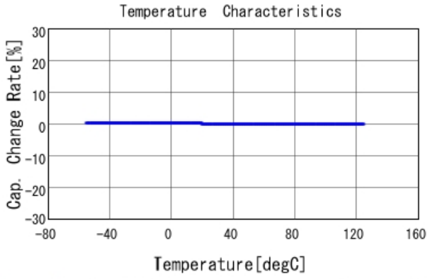
GRM3192C1H103JA01 C-Temp. capchange, DCOV, AC1Vrms
