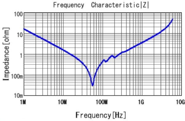
GRM3192C1H103JA01 |Z| DCOV, 20degC
