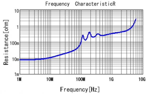
GRM3192C1H103JA01 R DCOV, 20degC
