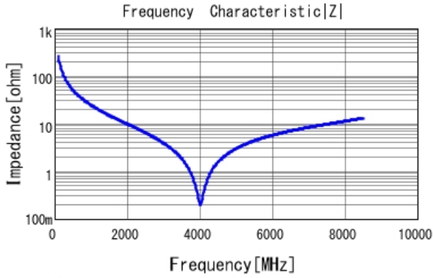
GJM0335C1E6R1BB01 |Z| DCOV, 25degC
