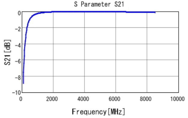
GJM0335C1E6R1BB01 S21 DCOV, 25degC
