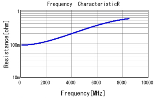
GJM0335C1E6R1BB01 R DCOV, 25degC
