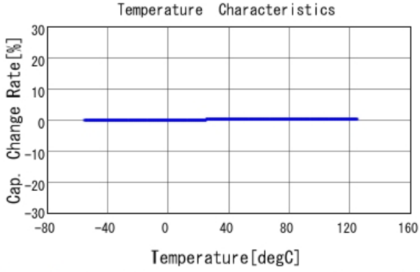
GJM0335C1E6R1BB01 C-Temp. capchange, DCOV, AC1Vrms
