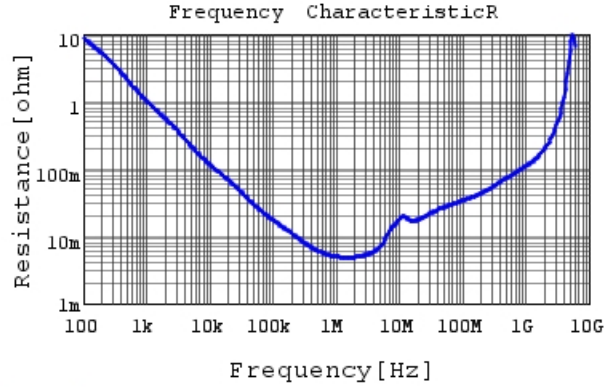
GRM219R6YA475MA73 R DCOV, 25degC
