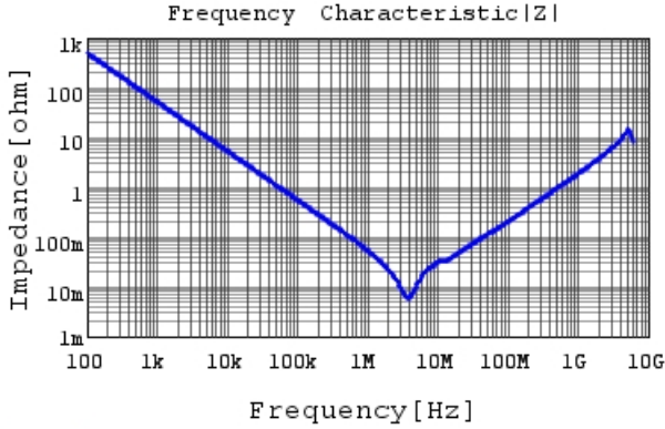
GRM219R6YA475MA73 |Z| DCOV, 25degC
