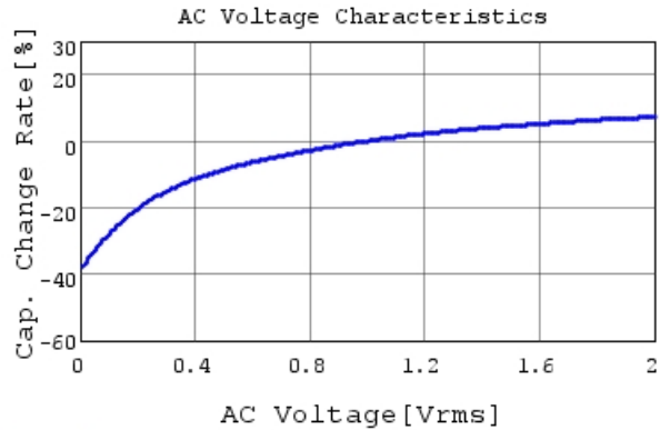
GRM219R6YA475MA73 C-AC Voltage capchange, DC
