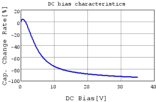
GRM219R6YA475MA73 C-DC bias capchange, 25.0c
