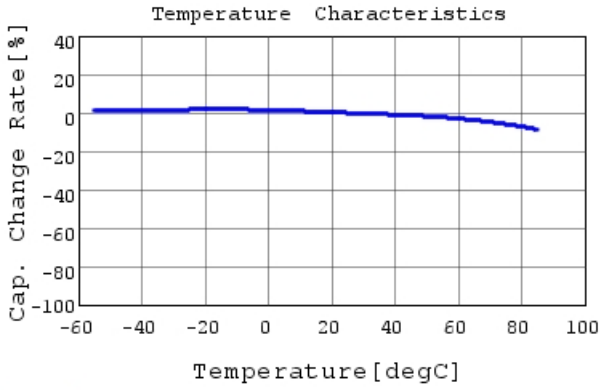
GRM219R6YA475MA73 C-Temp. capchange, DC0.0V,
