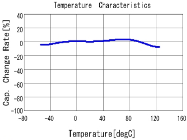
■ GRJ31CR71E106KE11 C-Temp. capchange, DC0.0V, AC1.0V r m
