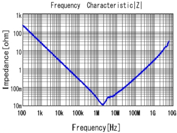
■ GRJ31CR71E106KE11 |Z| DCOV, 25degC
