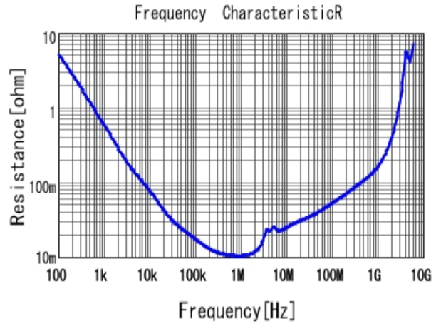
■ GRJ31CR71E106KE11 R DCOV, 25degC
