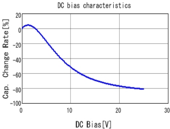
■ GRJ31CR71E106KE11 C-DC bias capchange, 25.0degC, AC1.
