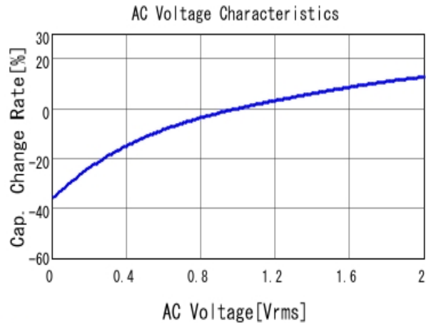
■ GRJ31CR71E106KE11 C-AC Voltage capchange, DCOV, 25.0d
