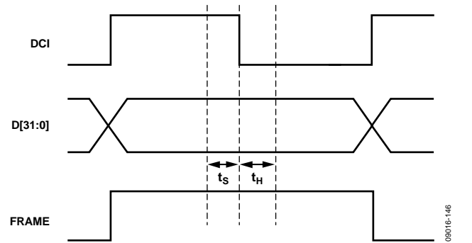
Figure 45. Timing Diagram for Input Data Ports
