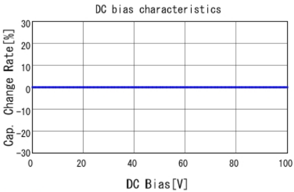
GCM3195C2A103JA16 C-DC bias capchange, 25.0degC, A
