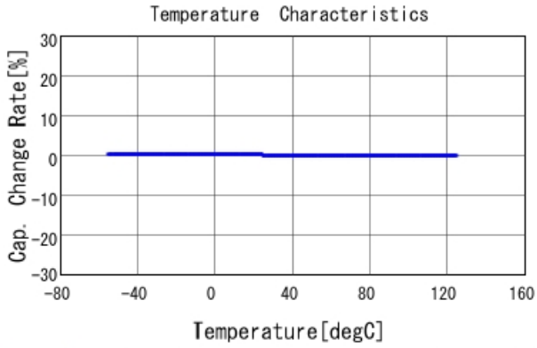
GCM3195C2A103JA16 C-Temp. capchange, DCOV, AC1Vrms
