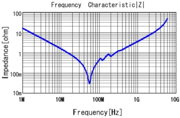
GCM3195C2A103JA16 |Z| DCOV, 25degC
