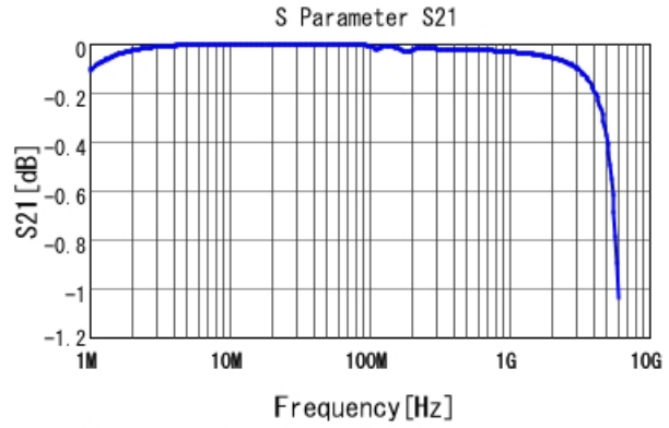
GCM3195C2A103JA16 S21 DCOV, 25degC
