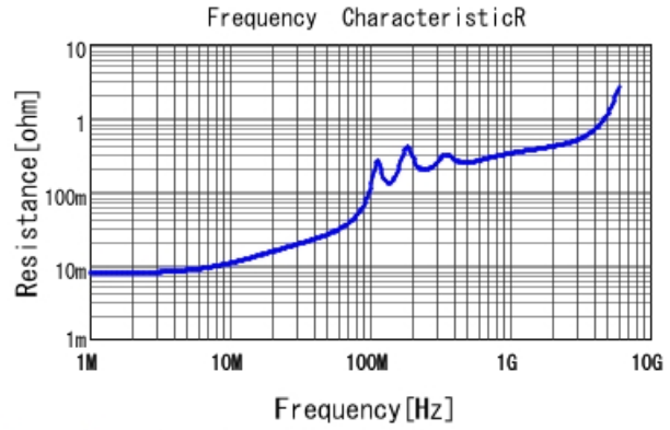
GCM3195C2A103JA16 R DCOV, 25degC
