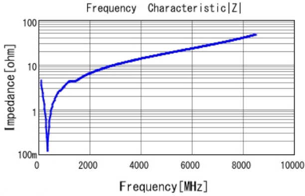
GRM1885C2A331JA01 |Z| DCOV, 25degC
