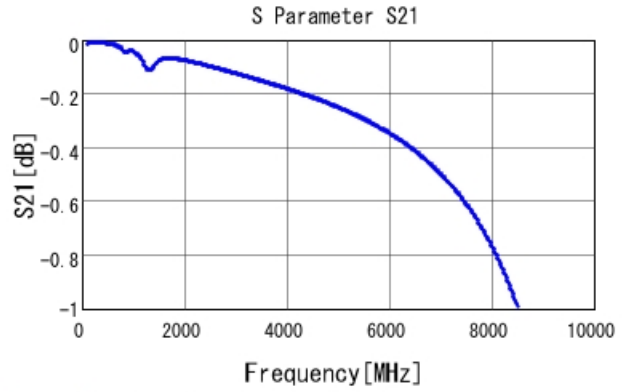
GRM1885C2A331JA01 S21 DCOV, 25degC
