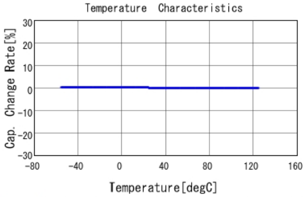
GRM1885C2A331JA01 C-Temp. capchange, DCOV, AC1Vrms
