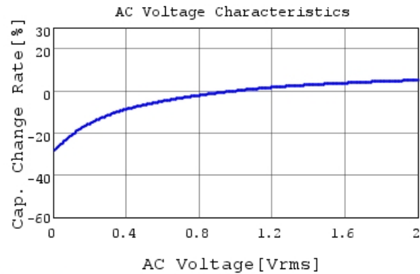
GRT188C81C475KE13 C-AC Voltage capchange, Dc
