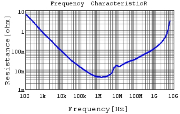
GRT188C81C475KE13 R DCOV, 25degC
