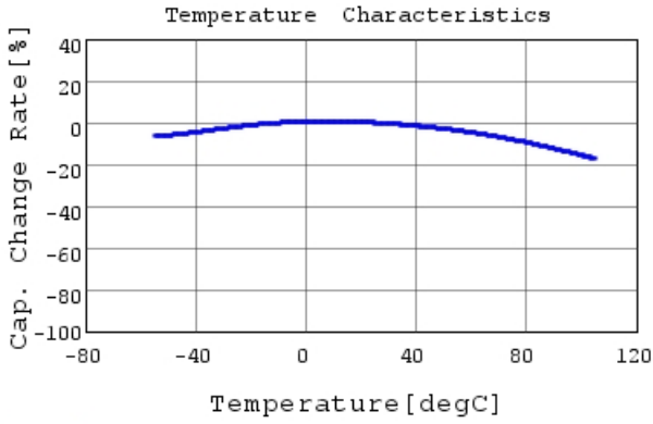
GRT188C81C475KE13 C-Temp. capchange, DC0.0V,
