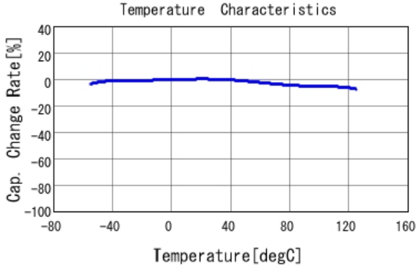
■ GCD188R72A682MA01 C-Temp. capchange, DCO. 0V, AC1. 0Vrm
