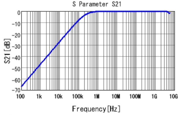
■ GCD188R72A682MA01 S21 DCOV, 25degC
