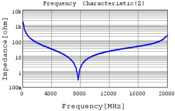
GCQ1555C1H1R0WB01 |Z| DCOV, 25degC
