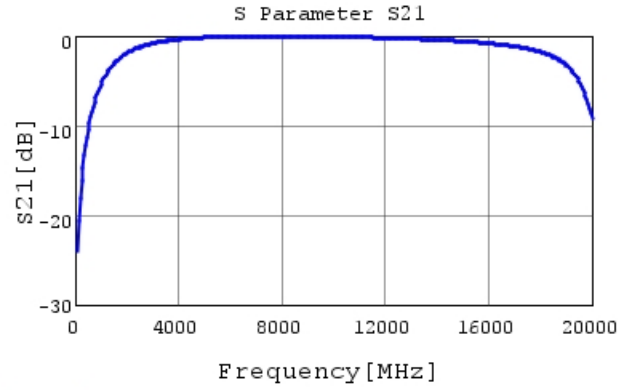
GCQ1555C1H1R0WB01 S21 DCOV, 25degC
