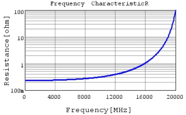
GCQ1555C1H1R0WB01 R DCOV, 25degC
