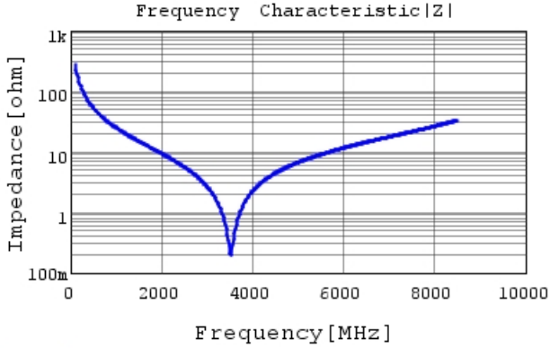
GCQ1555C1H5R9WB01 |Z| DC0V, 25degC
