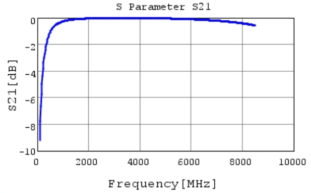
GCQ1555C1H5R9WB01 S21 DCOV, 25degC
