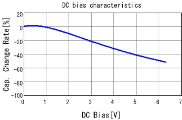
GRM32ER60J476KE64 C-DC bias capchange, 25.0degC, A
