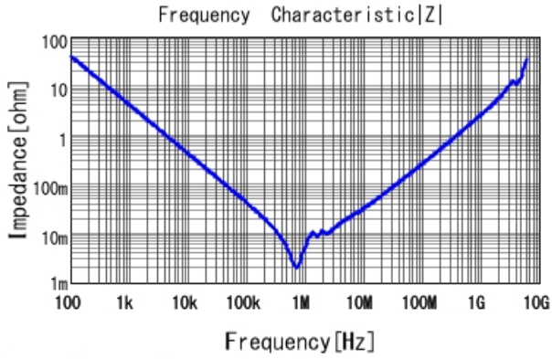
GRM32ER60J476KE64 |Z| DCOV, 25degC
