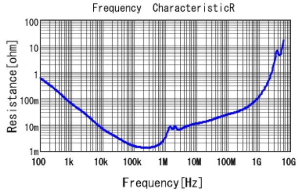
GRM32ER60J476KE64 R DCOV, 25degC
