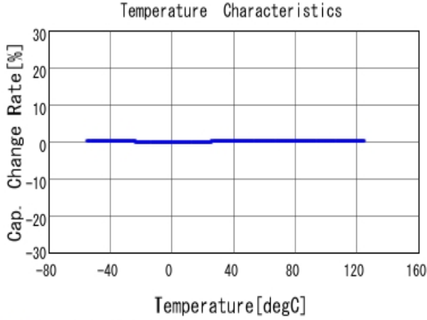
■ GQM2195C2E1R5BB12 C-Temp. capchange, DCOV, AC1Vrms
