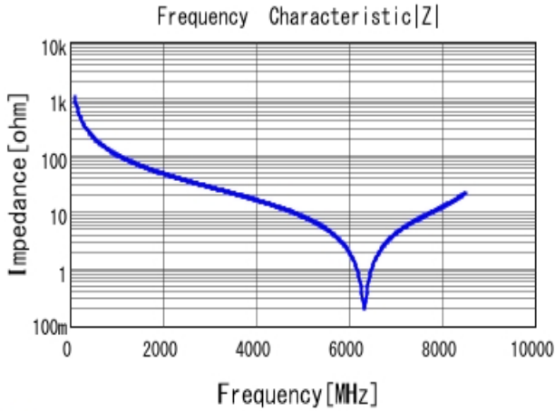
■ GQM2195C2E1R5BB12 |Z| DC0V, 25degC
