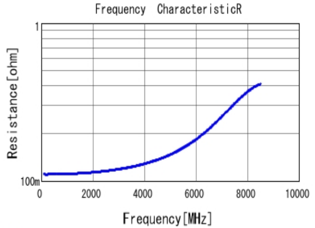
■ GQM2195C2E1R5BB12 R DC0V, 25degC
