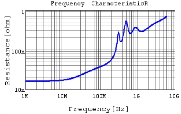
GRT1885C1H222JA02 R DCOV, 25degC
