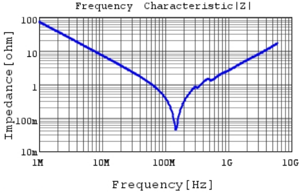
GRT1885C1H222JA02 |Z| DCOV, 25degC
