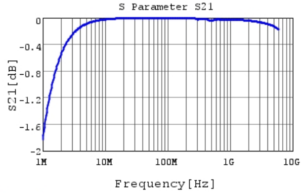
GRT1885C1H222JA02 S21 DCOV, 25degC
