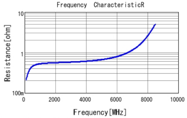
GRM1885C1H1R8CA01 R DCOV, 25degC
