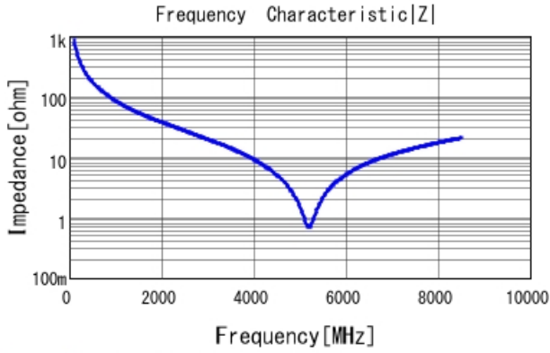
GRM1885C1H1R8CA01 |Z| DCOV, 25degC
