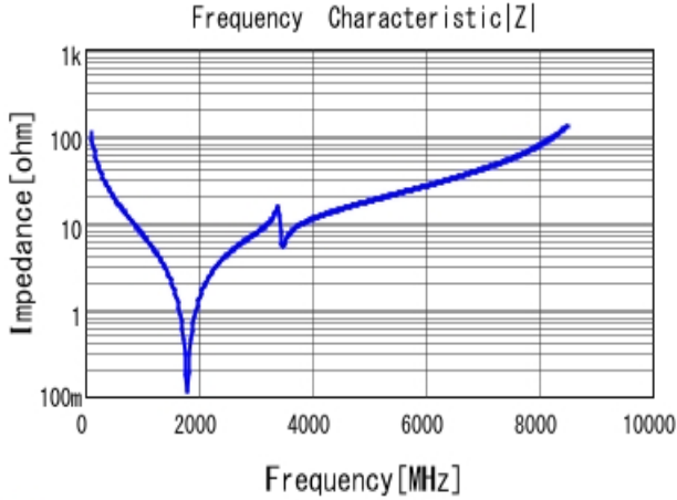
■ GQM1885C1H150JB01 |Z| DCOV, 25degC
