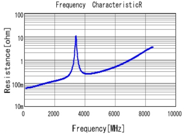
■ GQM1885C1H150JB01 R DCOV, 25degC
